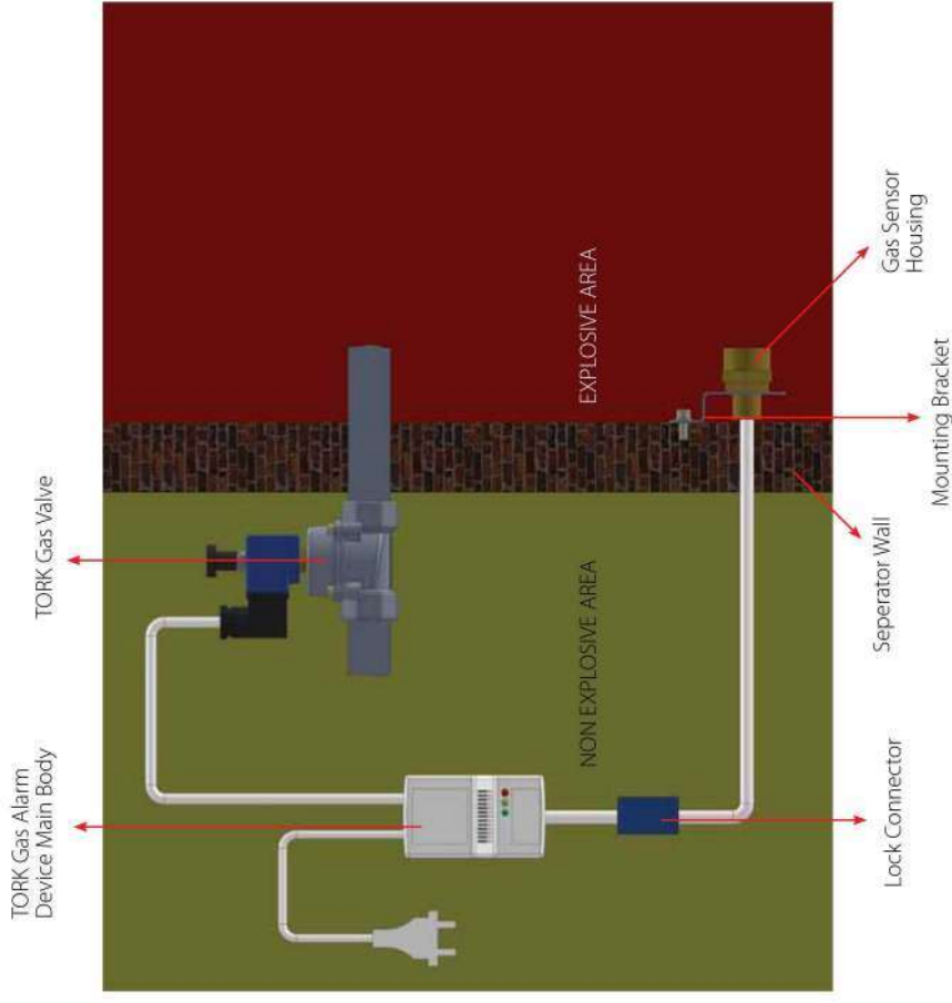
Fig 1. Installation of Gas Alarm Device with Ex Proof Sensor Housing
